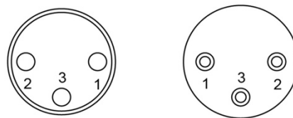
3 Pin XLR
