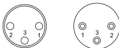
3 Pin XLR
